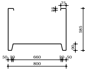
PB13.1 800x800x600
