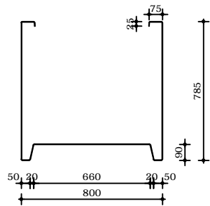
PB13 800x800x800
