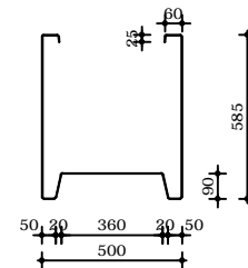
Dwarsdoorsnede PB23 1500x500x600
