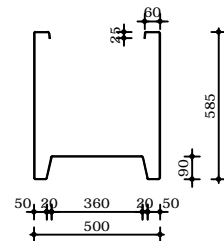
Dwarsdoorsnede PB24.1 900x500x600
