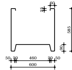
PB15 600x600x600
