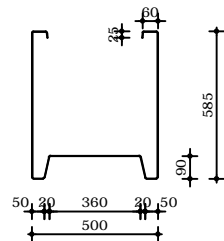
Dwarsdoorsnede PB22 2000x500x600
