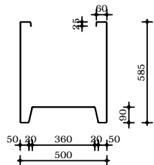
Dwarsdoorsnede PB24 1200x500x600
