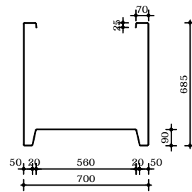
PB14 700x700x700
