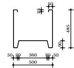
PB16 500x500x500
